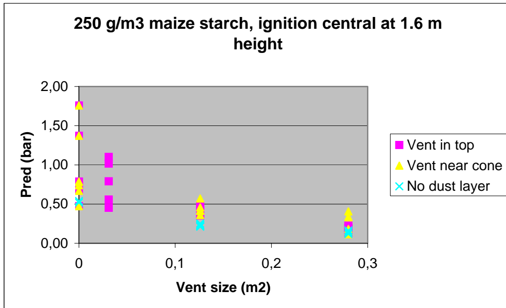
Figure 7 Venting experiments: effect of vent size, vent opening position, presence of dust layer on reduced overpressure in spray dryer (cloud of maize starch 250 g.m -3 in cone, ignition at 1.6 m height, static vent opening pressure P stat = 0.1 bar).
