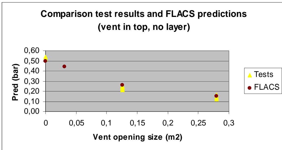
Figure 8 Effect of vent size (located in the top of the dryer) on maximum reduced overpressure. Comparison between predictions with CFD-tool FLACS and experiments (cloud of maize starch 250 g.m -3 in cone, ignition at 1.6 m height).
