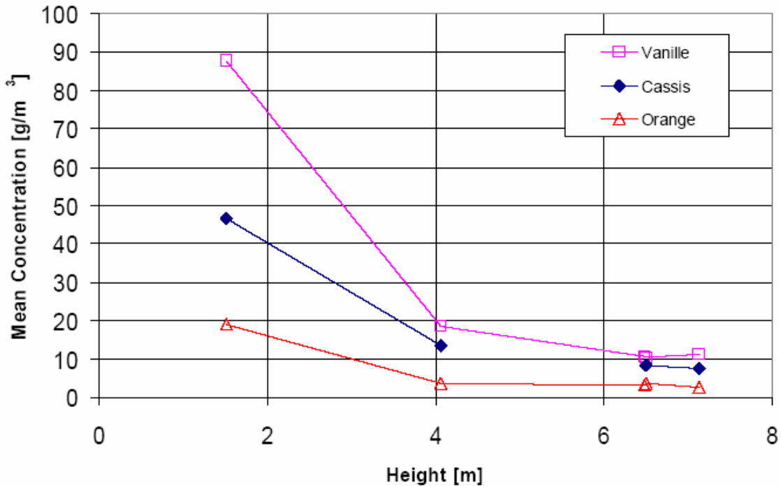
Figure 3 Measured mean concentration values as a function of the height (measured from the bottom) for three different products in a 132 m 3 spray dryer (conical bottom).
